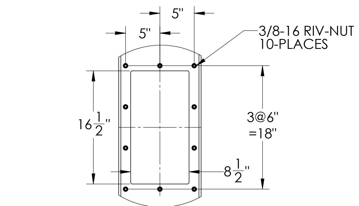
DISCHARGE FLANGE DETAIL B SCALE 1 : 8
