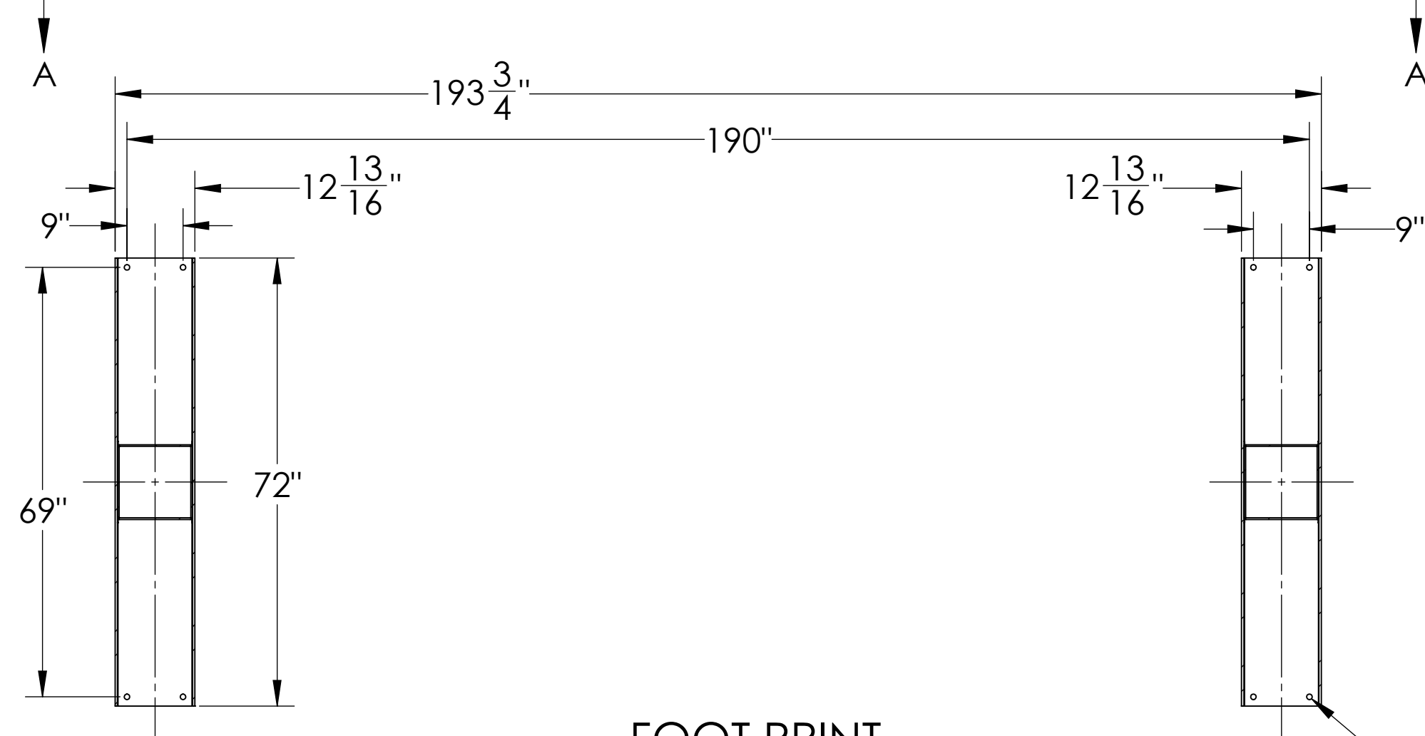
FOOT PRINT SECTION A-A
