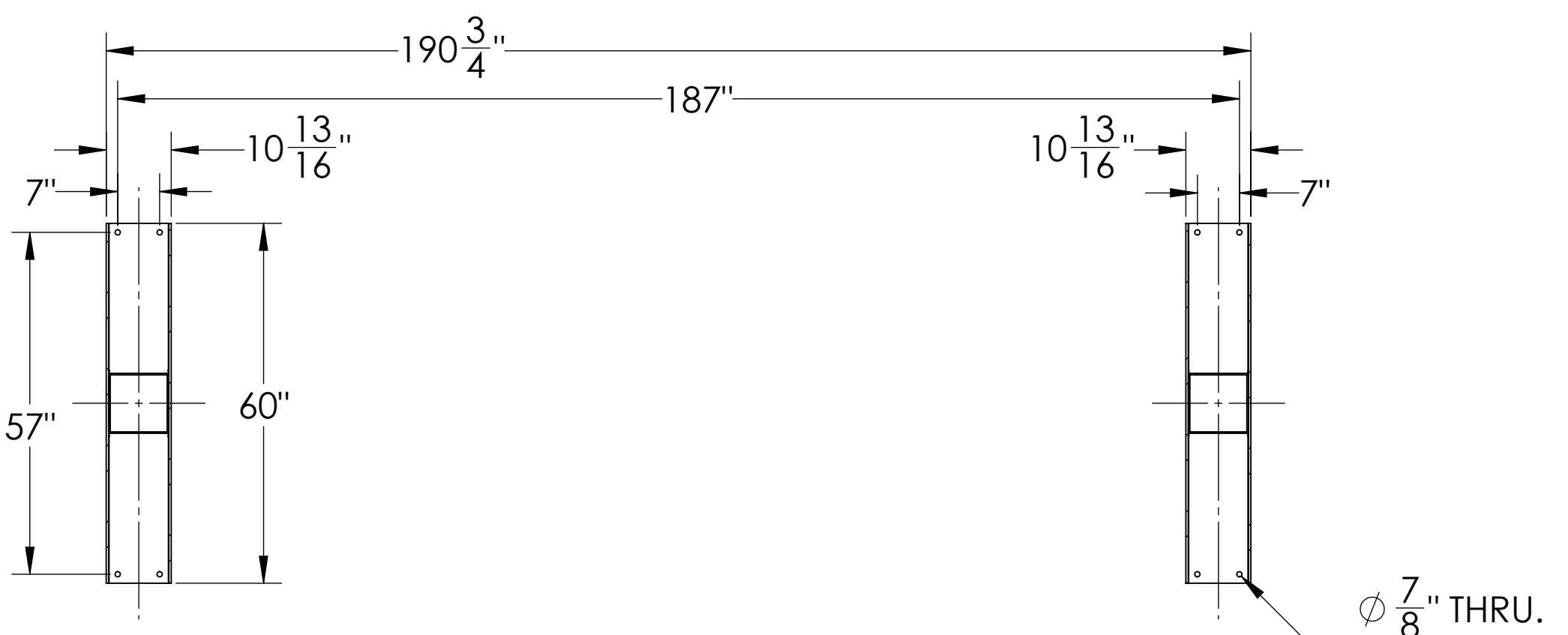
FOOT PRINT SECTION A-A
