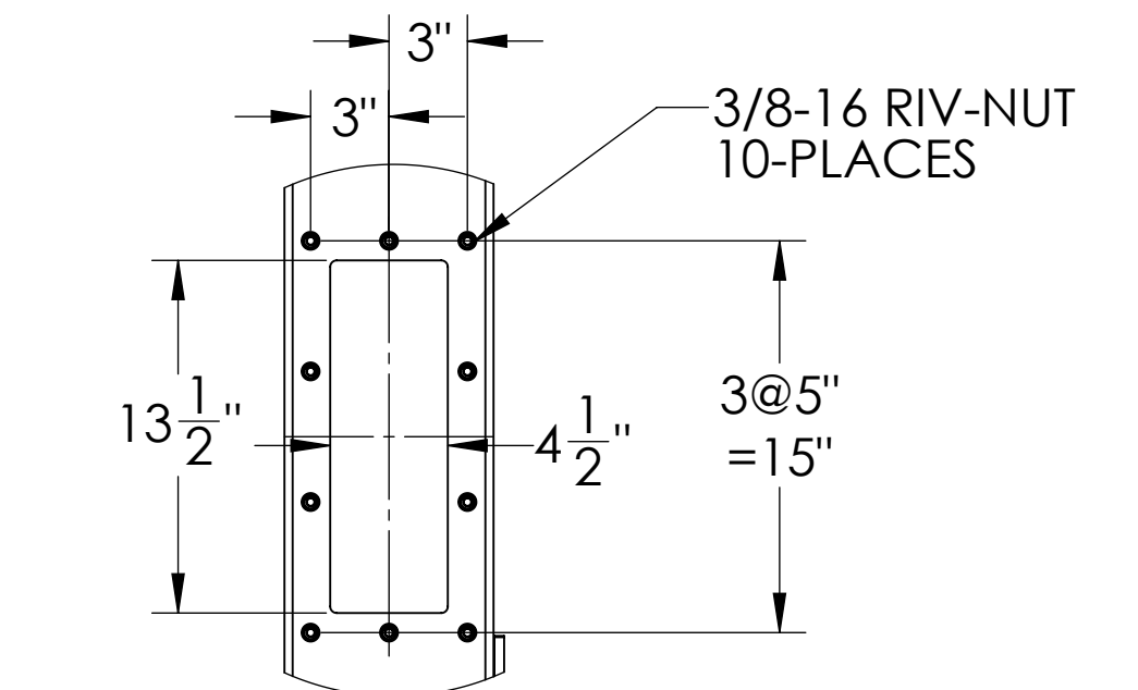
DISCHARGE FLANGE DETAIL B SCALE 1 : 8
