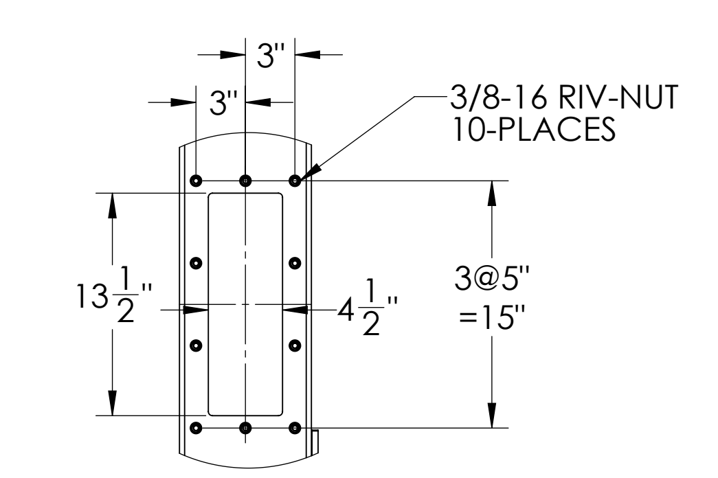
DISCHARGE FLANGE DETAIL B SCALE 1 : 8
