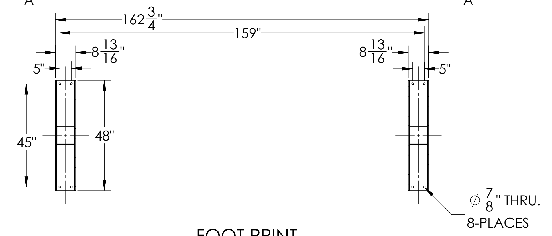
FOOT PRINT SECTION A-A
