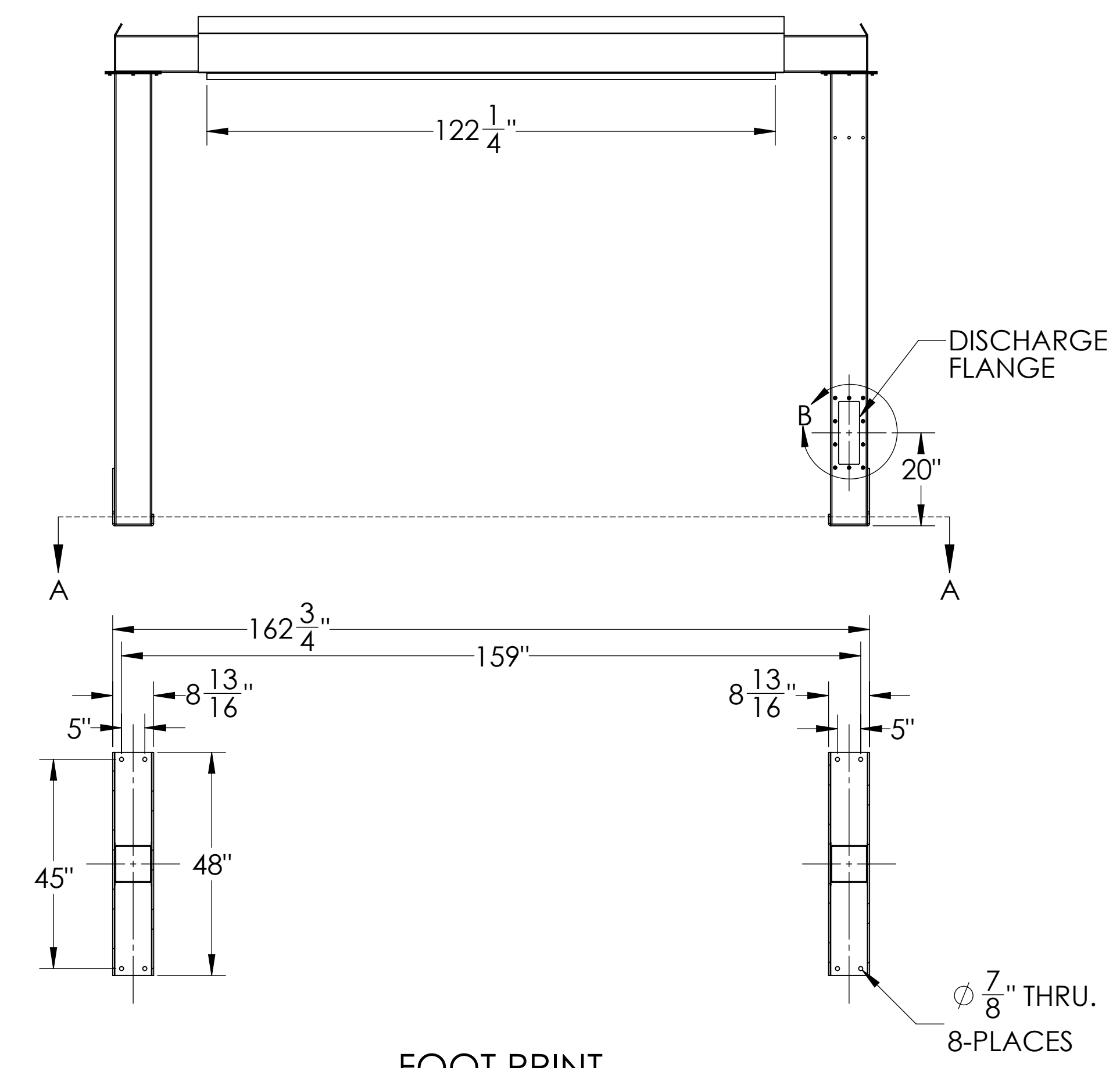
FOOT PRINT SECTION A-A
