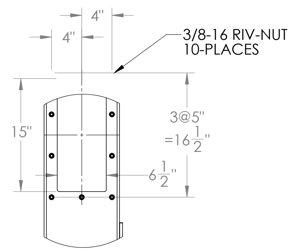
DISCHARGE FLANGE DETAIL B SCALE 1 : 8
