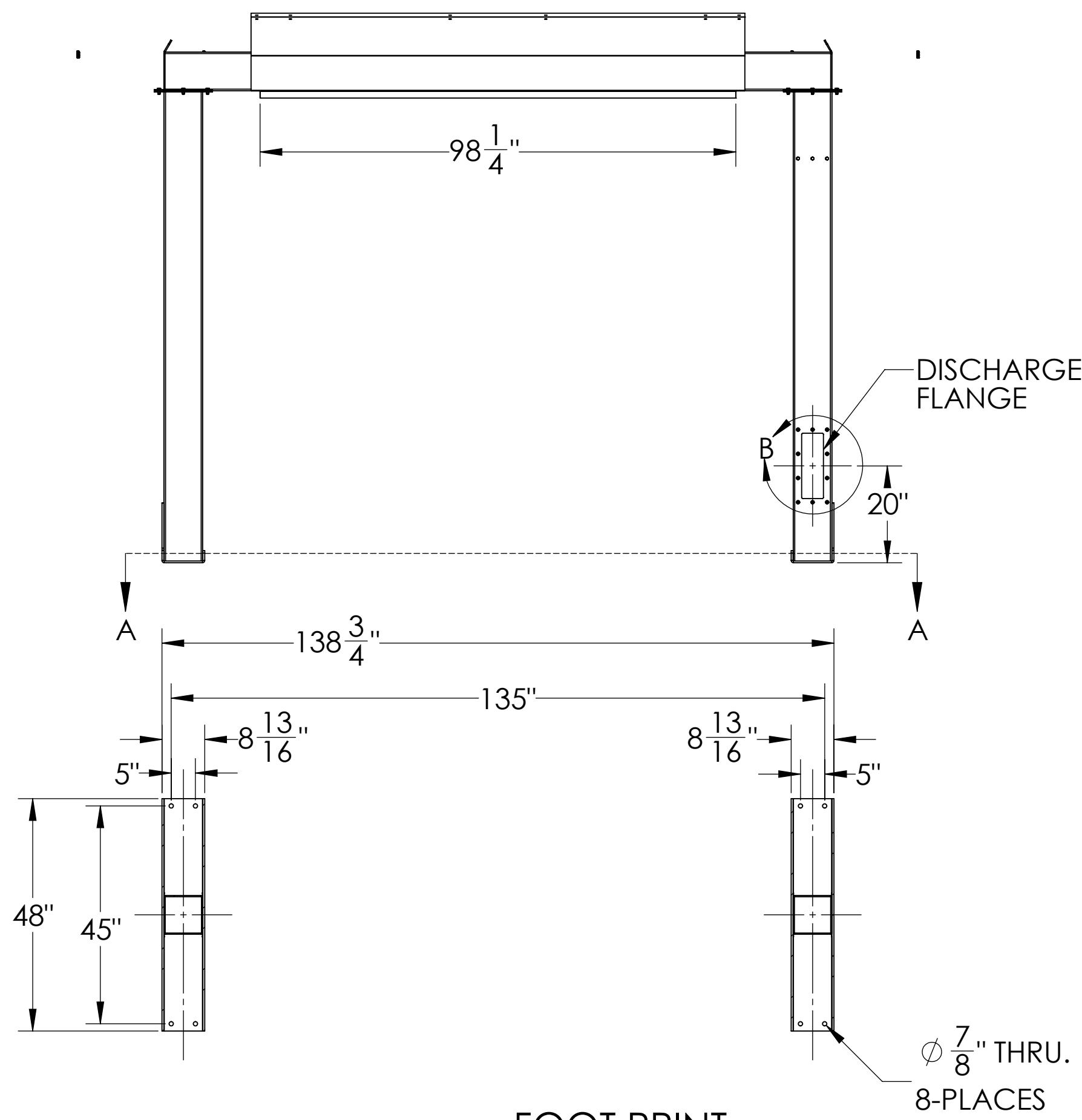
FOOT PRINT SECTION A-A
