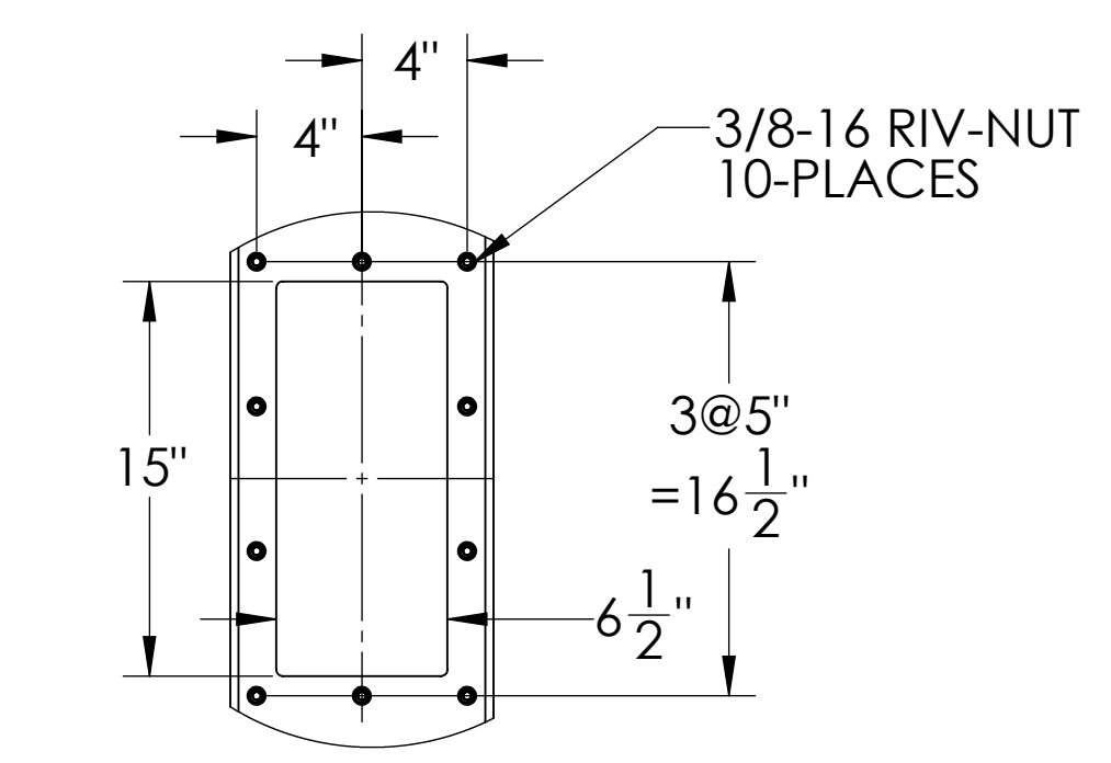
DISCHARGE FLANGE DETAIL B SCALE 1 : 8
